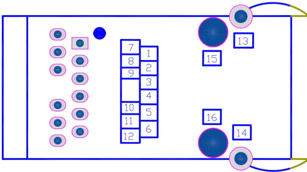
Diagram 4-2 pin diagram of K7(left for top view, right for bottom view)
